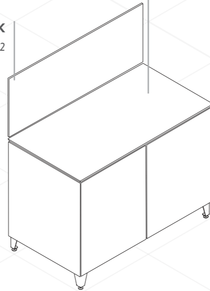
ADAPT 120 L 1200 x 700 x 900 Leg base
